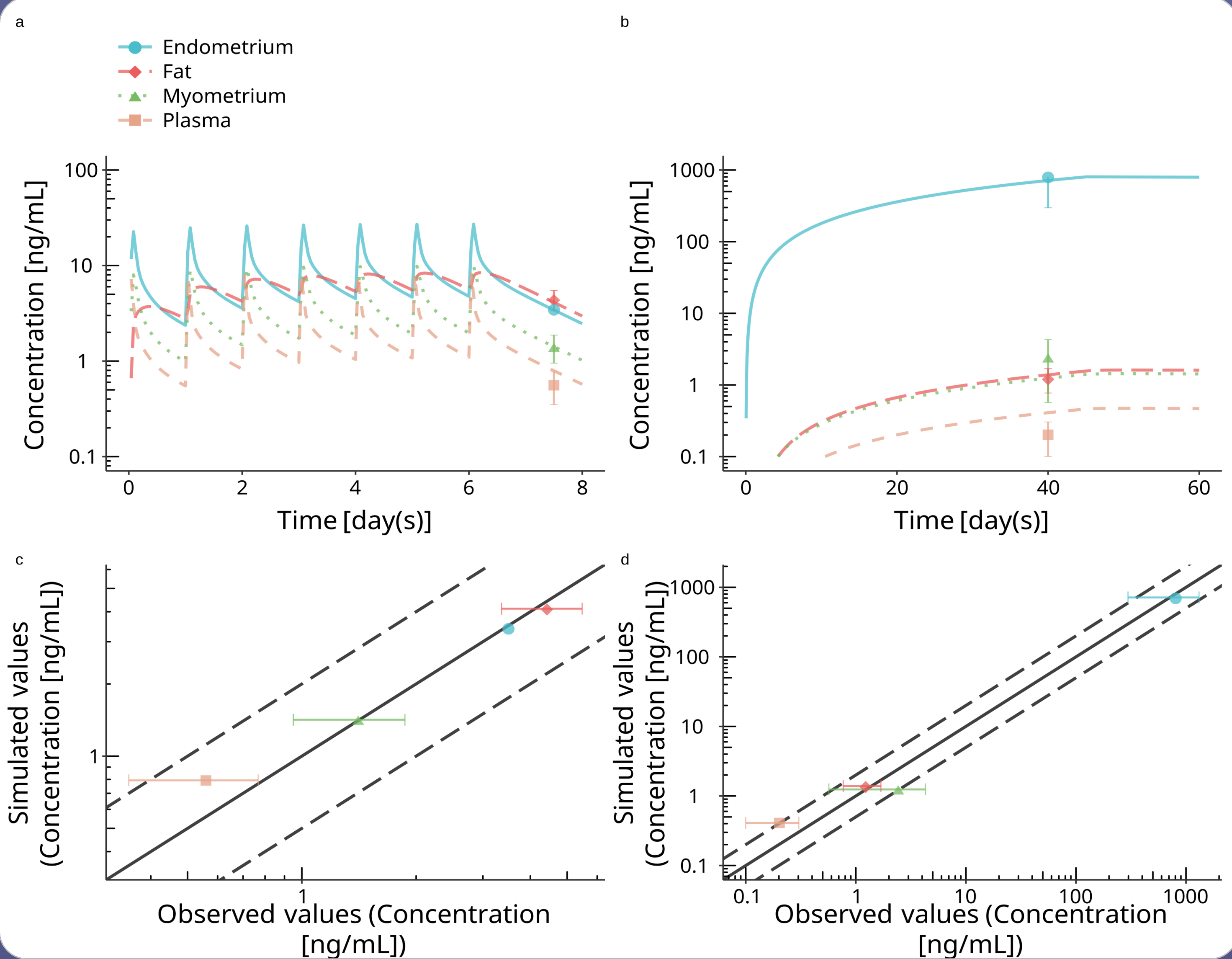
Figure 3: Plasma, fat, and uterine concentrations for oral and intrauterine (IUD) administration of levonorgestrel. Lines represent predicted concentration in endometrium (blue), fat (red), myometrium (green), and plasma (orange) for oral (a) and IUD (b) administration. Simulated versus observed data are shown for oral (c) and IUD (d) administration, with the line representing unity and dotted lines representing a 2-fold prediction error. Observed concentrations (mean \pm SD) are shown for endometrium (circle), fat (diamond), myometrium (triangle) and plasma (square) [8].
